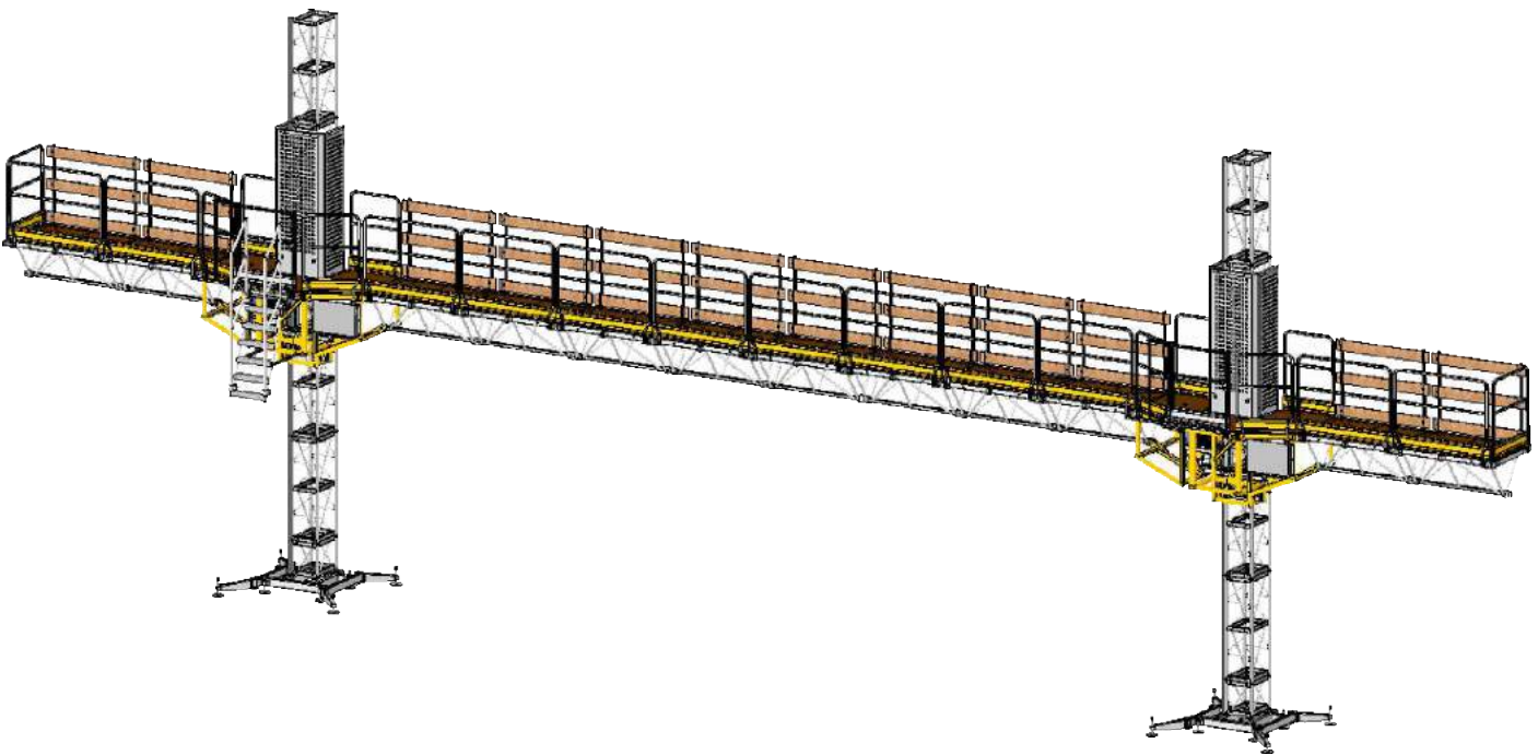
PIATTAFORMA AUTOSOLLEVANTE BICOLONNA ELSA P40/34 TWIN MAST CLIMBING WORK PLATFORM ELSA P40/34
