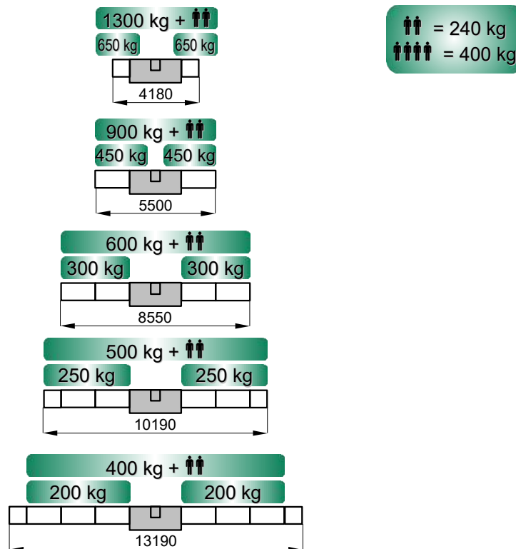
CARICHI MASSIMI ELSA P40/13 MAX LOADS ELSA P40/13
