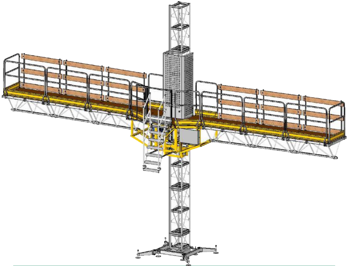
PIATTAFORMA AUTOSOLLEVANTE MONOCOLONNA ELSA P40/13 SINGLE MAST CLIMBING WORK PLATFORM ELSA P40/13
